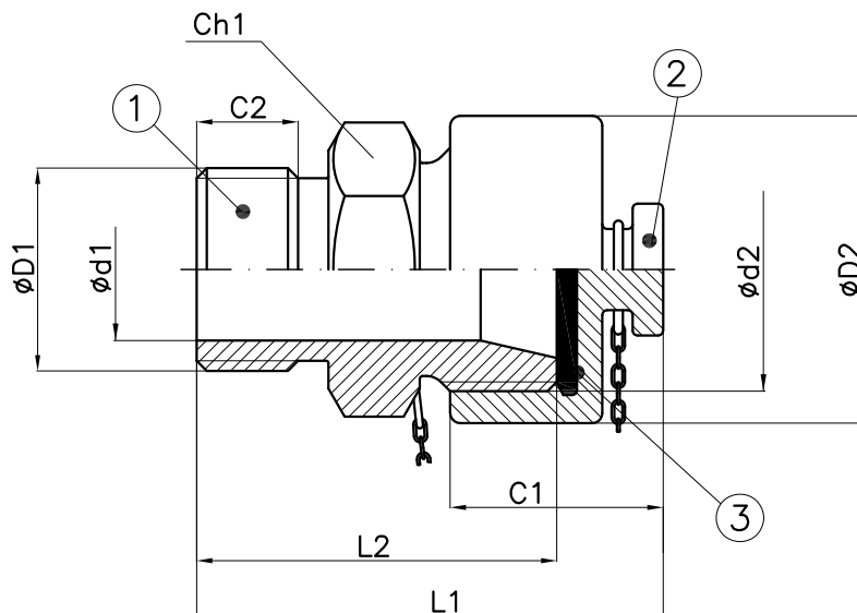
Attacchi per manichette Hose connection
